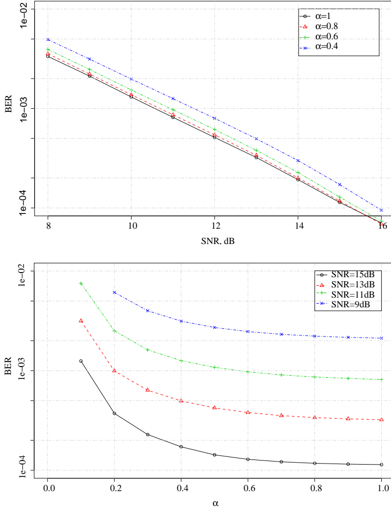
Figure 3: 1D slices of the configuration space \{c_k\}_{k=1}^M with fixed branch power imbalance factor \alpha = 10^{-0.1|S_1-S_2|} and varying effective SNR S = 10 \log_{10} ((10^{0.1S_1} + 10^{0.1S_2})/2) (top), and fixed effective SNR S and varying branch power imbalance factor \alpha (bottom). These slices were computed from the surface fit onto the data in Figure 2 (bottom). The entire fitted surface is shown in Figure 4.
