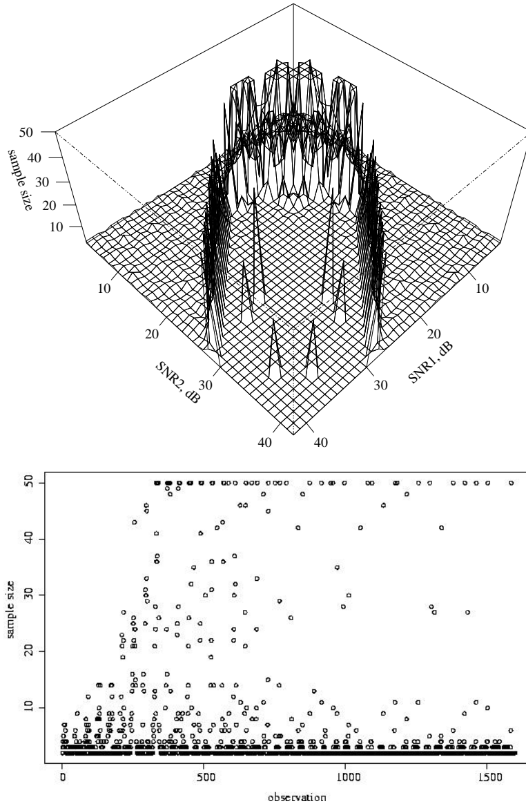
Figure 6: Sample sizes for Figure 2 (bottom). The top part shows the perspective plot and the bottom part shows the scatter plot.
