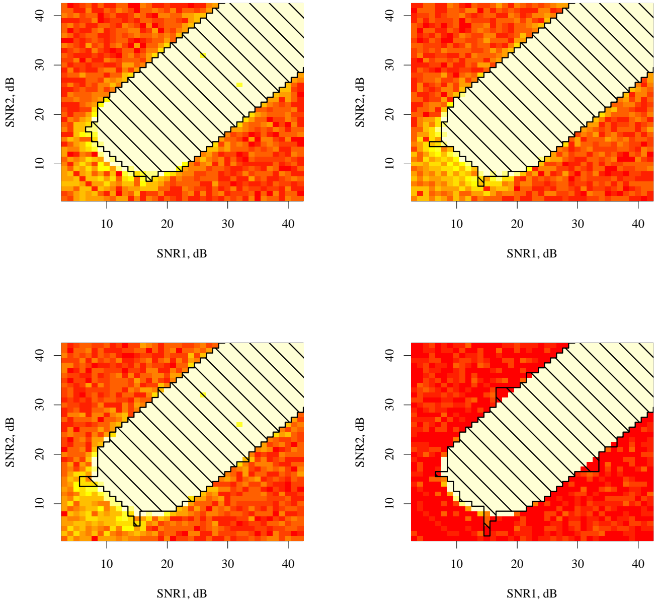
Figure 12: Cross-validation of optimized-support admissible regions with the confidence threshold \theta = 0.95 . The regions in top left, bottom left, and top right have been computed with n_k = 2 independent samples per bucket. There are 758 \pm 2 buckets (47% of all data) per such region. The region in the bottom right has been computed from the statistically significant data in Figure 2 (bottom). It consists of 766 buckets (48% of all data). Red (dark) corresponds to low bucket confidence and white (light) corresponds to high bucket confidence w.r.t. the voice quality threshold T = 10^{-3} .
