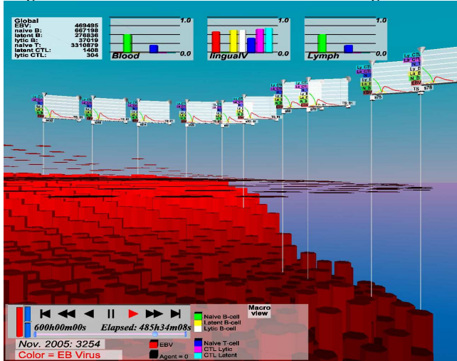
Figure 7: Dynamic PopView Annotations retrieved from the server
