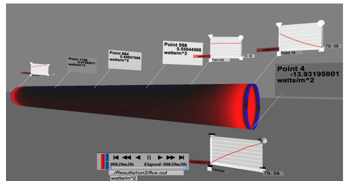
Figure 11: The result of adapting the IRVE-Serve system to space structure simulation with a linear color mapping
