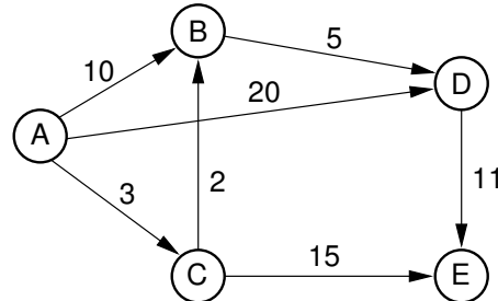
Figure 11.15 Example graph for shortest-path definitions.
