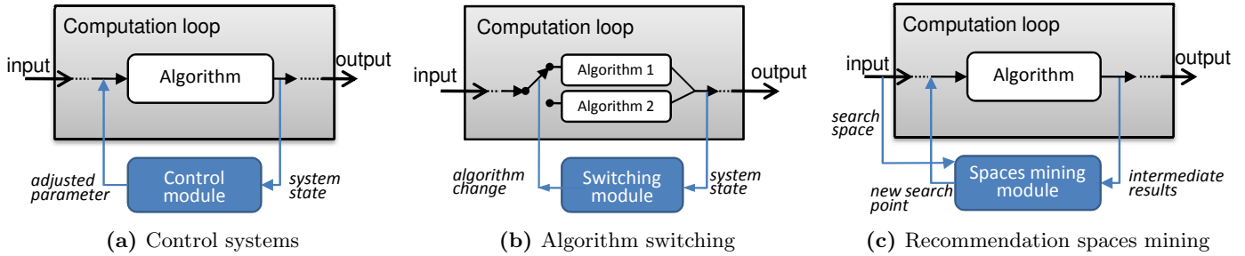
Figure 1: Adaptivity Schemas
