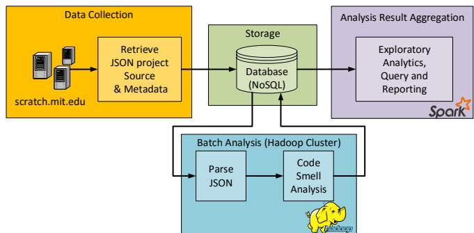
Fig. 1. Large-scale smell analysis infrastructure for block-based software.
