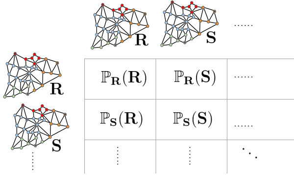
Fig. 6. Theoretically if the flip proposal is carried out sufficient number of times, one may approximate the stationary distribution of transitions of the state space, where each state correspond to a districting plan.
