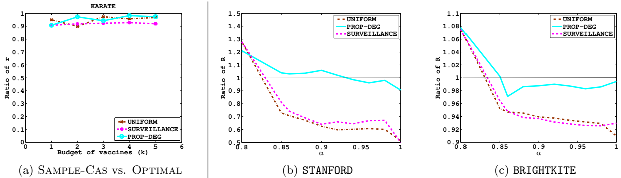
Figure 1: (a). Quality of Sample-Cas. Comparison between Sample-Cas and Optimal on KARATE over different distributions ( r = \frac{\# \text{healthy nodes saved by Sample-Cas}}{\# \text{healthy nodes saved by Optimal}} and \alpha = 0.5 ). (b) and (c). Comparison between Expect-Dom and Expect-Eig. Ratio of R ( R = \frac{\# \text{healthy nodes saved by Expect-Dom}}{\# \text{healthy nodes saved by Expect-Eig}} ) vs. \alpha . Expect-Dom performs better than Expect-Eig when R > 1 , otherwise Expect-Eig is better.
