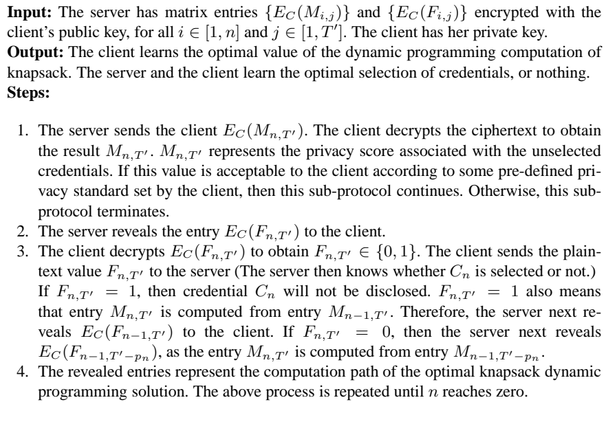
Fig. 2. Basic traceback sub-protocol
