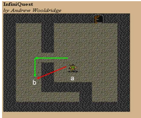
Fig. 1. Walking through walls: an example of semantic integrity violation. The central game server only keeps the coordinates of the two end points of a moving player as part of the abstract state, point a at (x_1, y_1) and point b at (x_2, y_2) . A cheating player may violate the game rules by walking through walls (the red path) without being detected by the state server.
