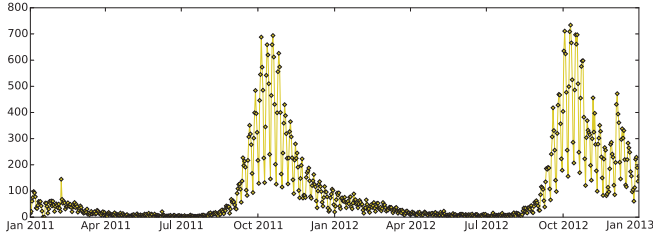
Figure 3: Counts of Twitter users in Virginia who got flu shot
