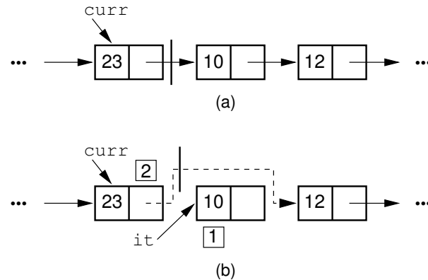
Figure 4.10 The linked list removal process. (a) The linked list before removing the node with value 10. (b) The linked list after removal. 1 marks the list node being removed. it is set to point to the element. 2 marks the next field of the preceding list node, which is set to point to the node following the one being deleted.
