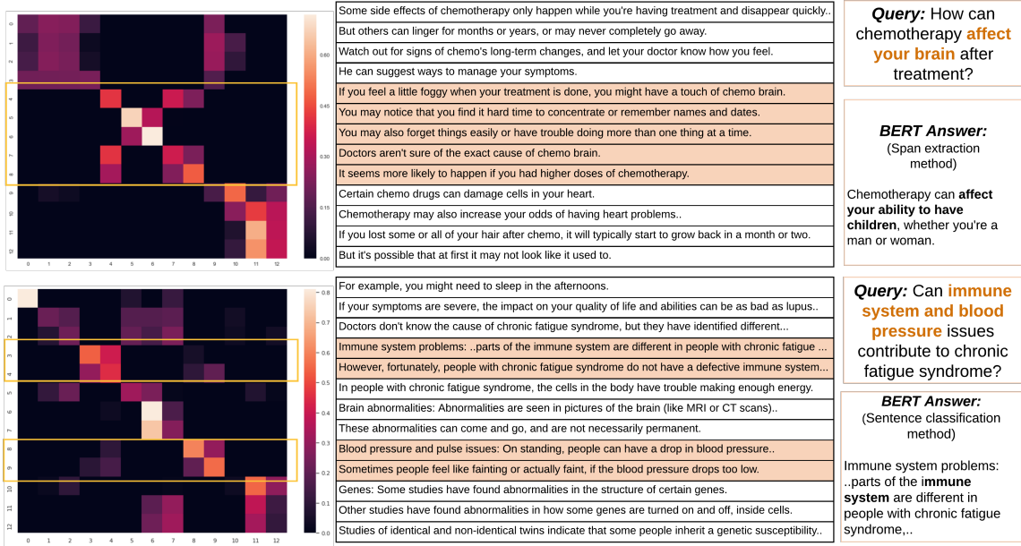
Figure 3: Heatmap of attention weights from the inter-sentence attention layer for two QA pairs. The matrices show the attention weights of each sentence with respect to every other sentence from the context. The high values of diagonal elements represent the weight of a sentence with respect to itself. Answers from BERT are shown on the right.
