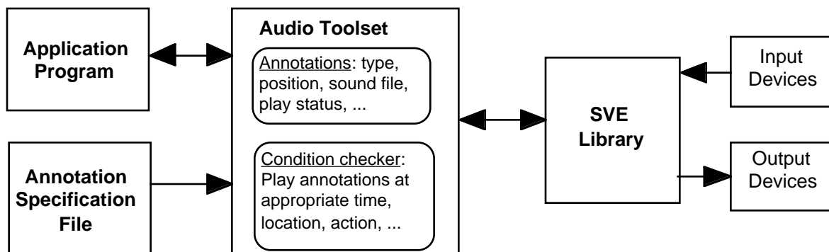
Figure 3. Structure of audio annotation toolset and related components.
