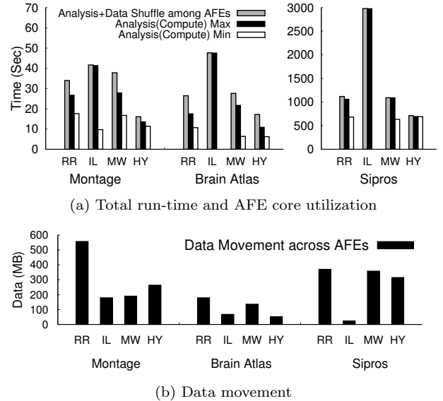
Figure 7: Performance of scheduling heuristics.
