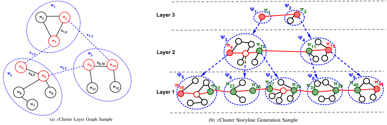
Fig. 4. \varepsilon Cluster algorithm sample. (a) shows a sample layer of an \varepsilon Cluster hierarchy; (b) depicts a story generation sample based on a three-layer \varepsilon Cluster hierarchy.
