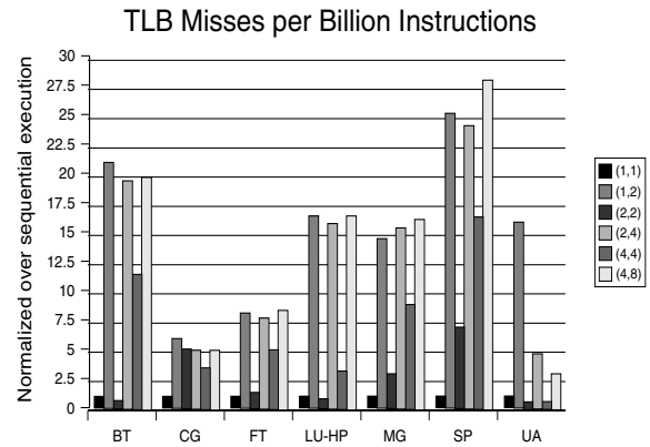
Figure 3. Normalized number of data TLB misses of the benchmarks per billion instructions executed.
