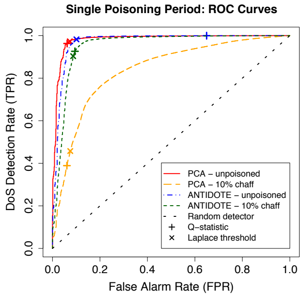
Figure 8: ROC curves of ANTIDOTE under Single-Training Period poisoning attacks.
