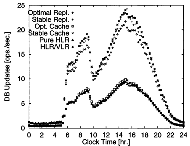
Figure 8. System-wide database updates.
