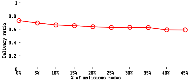
Figure 3: Delivery Ratio under Best Trust Formation.
