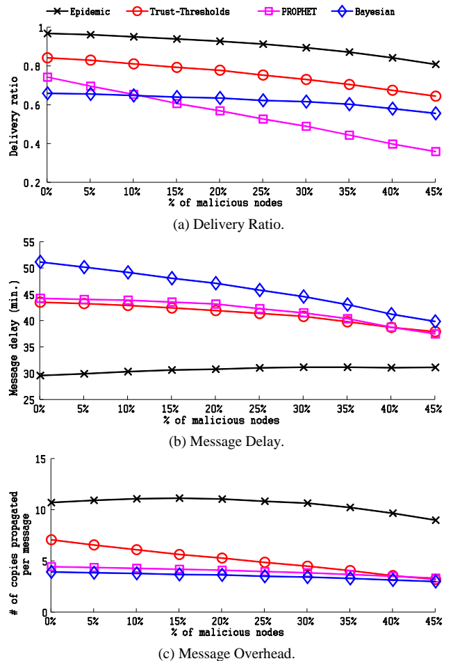
Figure 5: Performance Comparison (Analytical Results based on SWIM Mobility).
