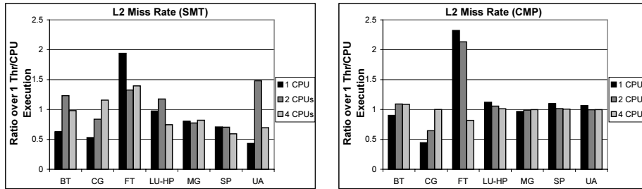
Fig. 1. Normalized L2 miss rates of the benchmarks on the SMT and CMP multiprocessor (left and right diagrams respectively). The corresponding 1 thread/processor miss rates on each architecture and number of processors have been used as references for the normalization.
