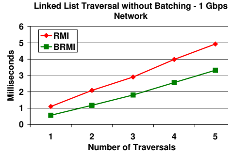
Figure 2: Linked List Traversal (Batches Size 1)
