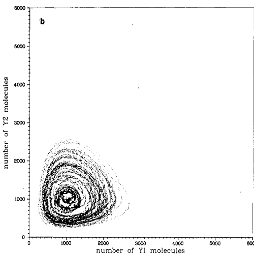
Figure 12. Results of a 1.5 \times 10^6 reaction stochastic simulation run of the Lotka reactions including reaction 38d, with c_1 = 0.0002 , c_2 = 0.01 , c_3 = c_4 = 10 , and X = 10^5 (constant), corresponding to the deterministic steady-state Y_1 = Y_2 = 1000 . (a) A 200 rpd plot of Y_1 vs. t for 0 \leq t \leq 30 . (b) A 200 rpd plot of Y_2 vs. Y_1 for 0 \leq t \leq 30 .
