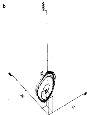
Figure 28. Same as Figures 24a and 24c, except that \rho_{1s} = 2000 and \rho_{2s} = 20000 .
