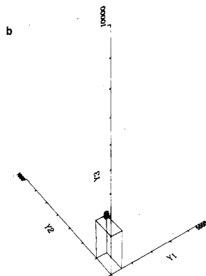
Figure 30. Same as Figures 24a and 24c, except that \rho_1 = 5000 and \rho_2 = 5000 .
