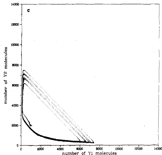
Figure 19. Same as Figure 18, except \alpha = 0.2 (corresponding to the same reaction parameters as for the runs in Figure 14).
