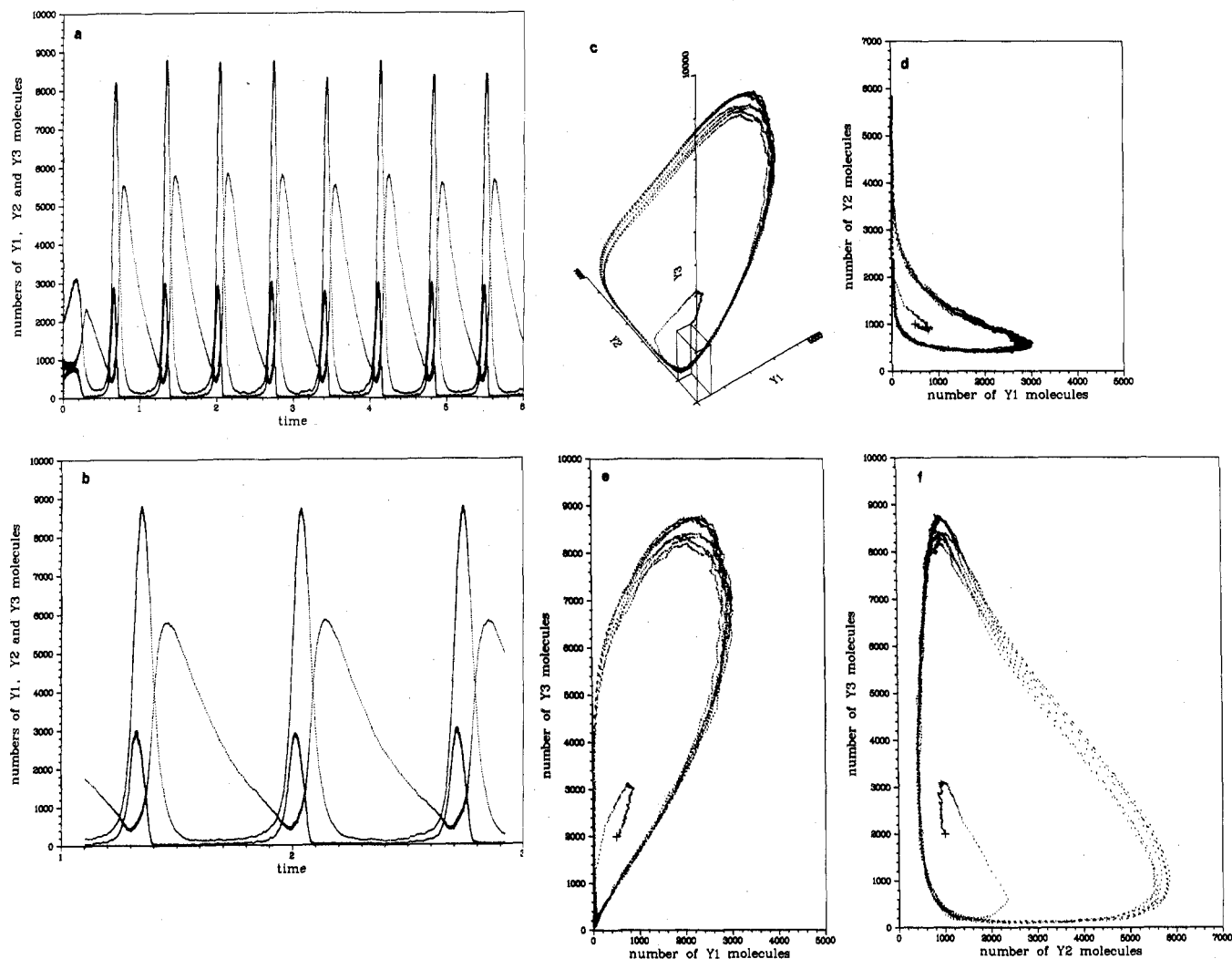
Figure 24. Results of a 0.71 \times 10^6 reaction stochastic simulation run of the Oregonator reactions (59), with Y_{1s} = 500 , Y_{2s} = 1000 , Y_{3s} = 2000 , \sigma_{1s} = 2000 , and \sigma_{2s} = 50000 [see (61)]. (a) Combined 100 rpd plots of Y_1 (low-peaking curve), Y_2 (middle-peaking curve), and Y_3 (high-peaking curve) vs. t for 0 \leq t \leq 6 . (b) Same as (a), but for 1 < t < 3 . (c) A 250 rpd plot in Y_1 Y_2 Y_3 space for 0 \leq t \leq 6 . (d) Projection of the trajectory in (c) onto the Y_1 Y_2 plane. (e) Projection of the trajectory in (c) onto the Y_1 Y_3 plane. (f) Projection of the trajectory in (c) onto the Y_2 Y_3 plane.
