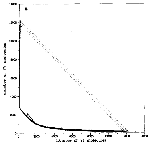
Figure 18. Results of a stochastic simulation run of the Brusselator with c_1 X_1 = 5000 , Y_{1_0} = 1000 , Y_{2_0} = 2000 , and \alpha = 0.1 , all plotted at 100 rpd: (a) Y_1 vs. t ; (b) Y_2 vs. t ; (c) Y_2 vs. Y_1 .
