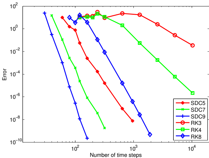
Figure 6. Error versus time step: serial Runge–Kutta and SDC methods for the Lorenz equation.
