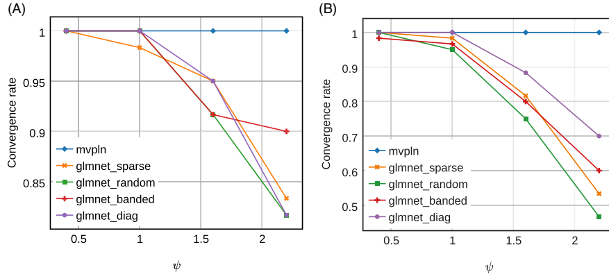
FIGURE 4 Convergence ratio of univariate Lasso regularized Poisson regression model (GLMNET) and multivariate Poisson log-normal (MVPLN) model when p < n (A) and p \geq n (B). Since MVPLN model always converges, we use a single line to represent these 4 scenarios
