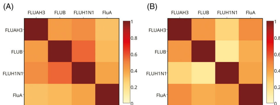
FIGURE 6 Heatmap of the averaged partial correlation matrix estimated by the multivariate Poisson log-normal (MVPLN) model for the one-step-ahead predictions on the real influenza-like-illness (ILI) datasets of Brazil (A) and Chile (B)
