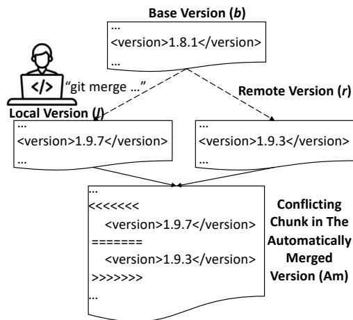
Figure 3: A conflict reported by git-merge
