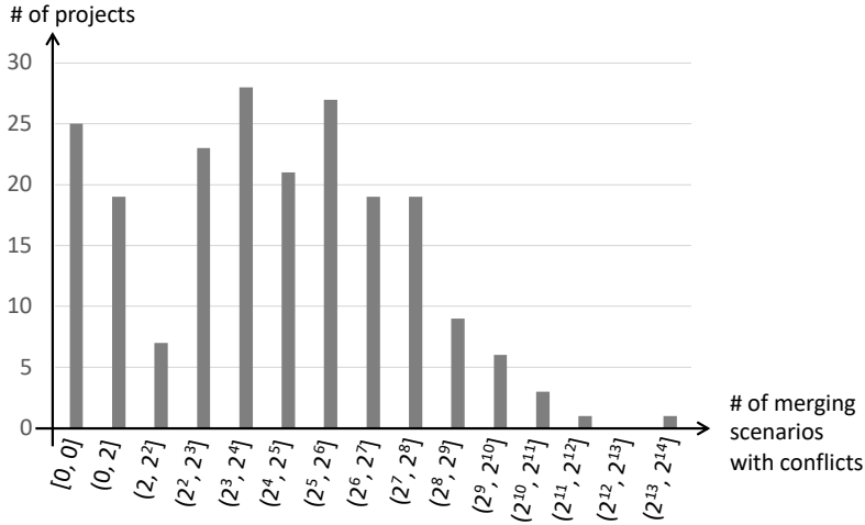
Figure 6: Project distribution based on the number of merging scenarios with conflicts
