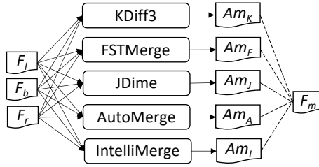
Figure 8: The experiment settings. Here, F_l , F_b , F_r , and F_m are folders to separately hold programs of local, base, remote, and manually merged versions. Am_K , Am_F , Am_J , Am_A , and Am_I are automatically merged versions separately produced by KDiff3, FSTMerge, JDime, AutoMerge, and IntelliMerge.
