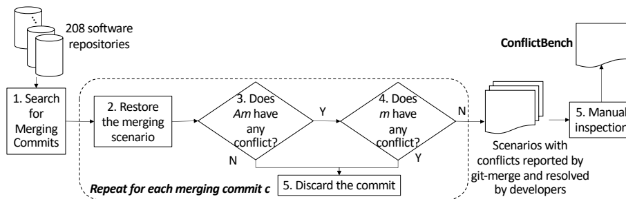
Figure 5: Our crawling process takes five steps to identify conflict samples
