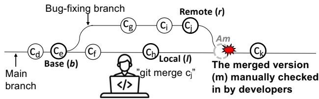
Figure 2: Text-based merge tools (e.g., git-merge) can be used to merge software branches and reveal conflicts
