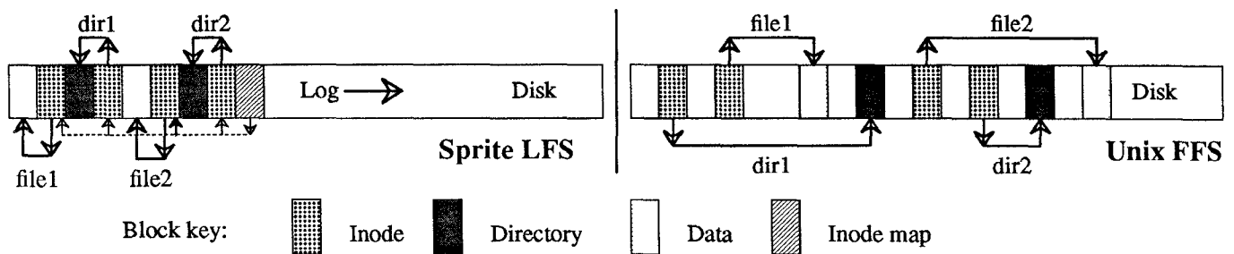
Figure 1 — A comparison between Sprite LFS and Unix FFS. This example shows the modified disk blocks written by Sprite LFS and Unix FFS when creating two single-block files named dir1/file1 and dir2/file2 . Each system must write new data blocks and inodes for file1 and file2 , plus new data blocks and inodes for the containing directories. Unix FFS requires ten non-sequential writes for the new information (the inodes for the new files are each written twice to ease recovery from crashes), while Sprite LFS performs the operations in a single large write. The same number of disk accesses will be required to read the files in the two systems. Sprite LFS also writes out new inode map blocks to record the new inode locations.
