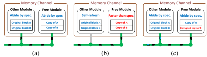
Fig. 8: (a) Write Mode under Hetero-DMR. (b) Read Mode under Hetero-DMR. (c) Error correction under Hetero-DMR.
