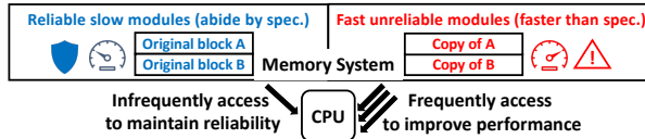
Fig. 7: Hetero-DMR overview.
