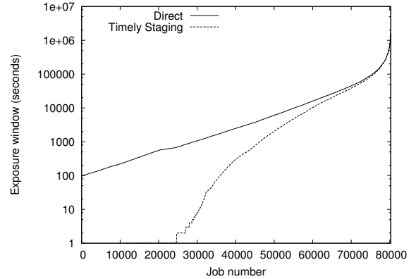
Figure 9. Size of exposure window for each job in the log.
