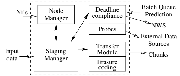
Figure 3. Implementation architecture for timely staging.
