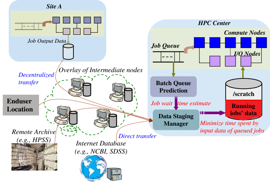
Figure 1. Overview of the timely staging framework, and interactions between the components.
