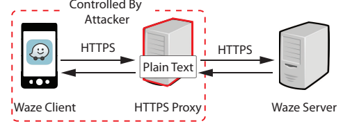
Figure 4: Using a HTTPS proxy as man-in-the-middle to intercept traffic between Waze client and server.
