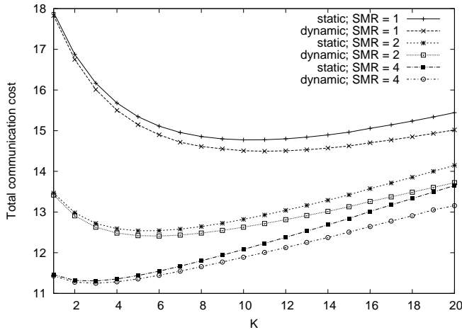
Fig. 6. Total communication cost vs. K .
