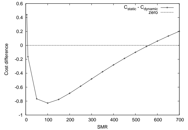
Fig. 7. C_{static} - C_{dynamic} vs. SMR.
