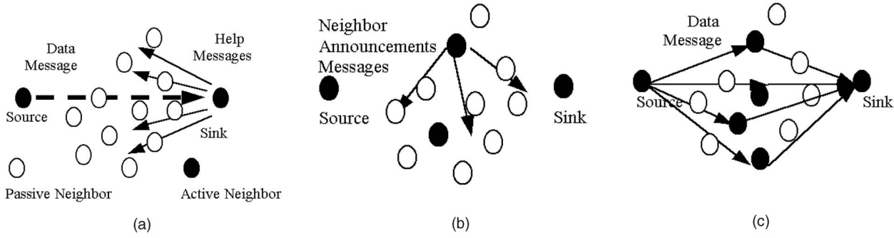
Fig. 1. Network self-configuration example. (a) Communication hole. (b) Transition. (c) Final state.
