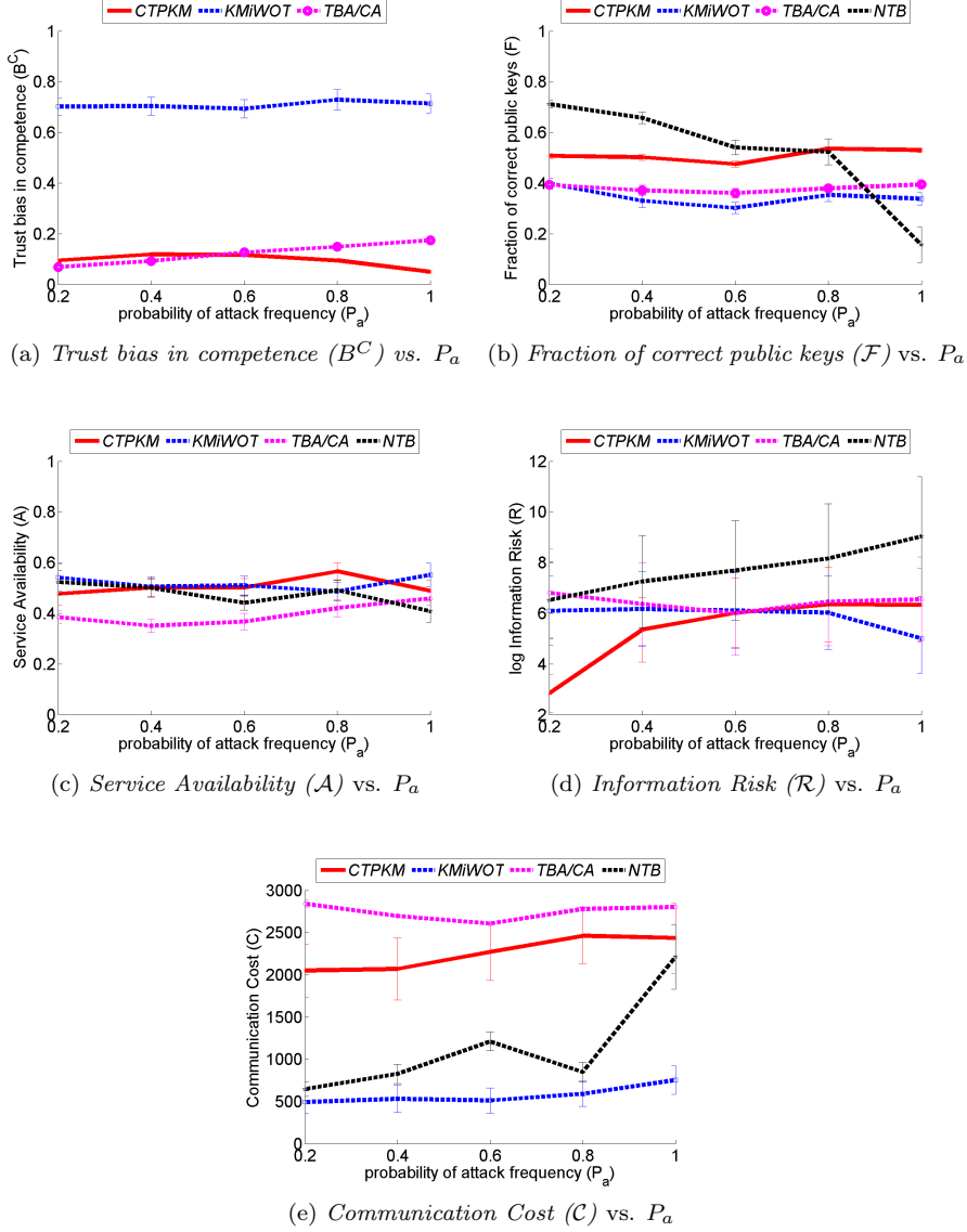
Figure 4: Effect of attack intensity ( P_a ) on trust bias and performance
