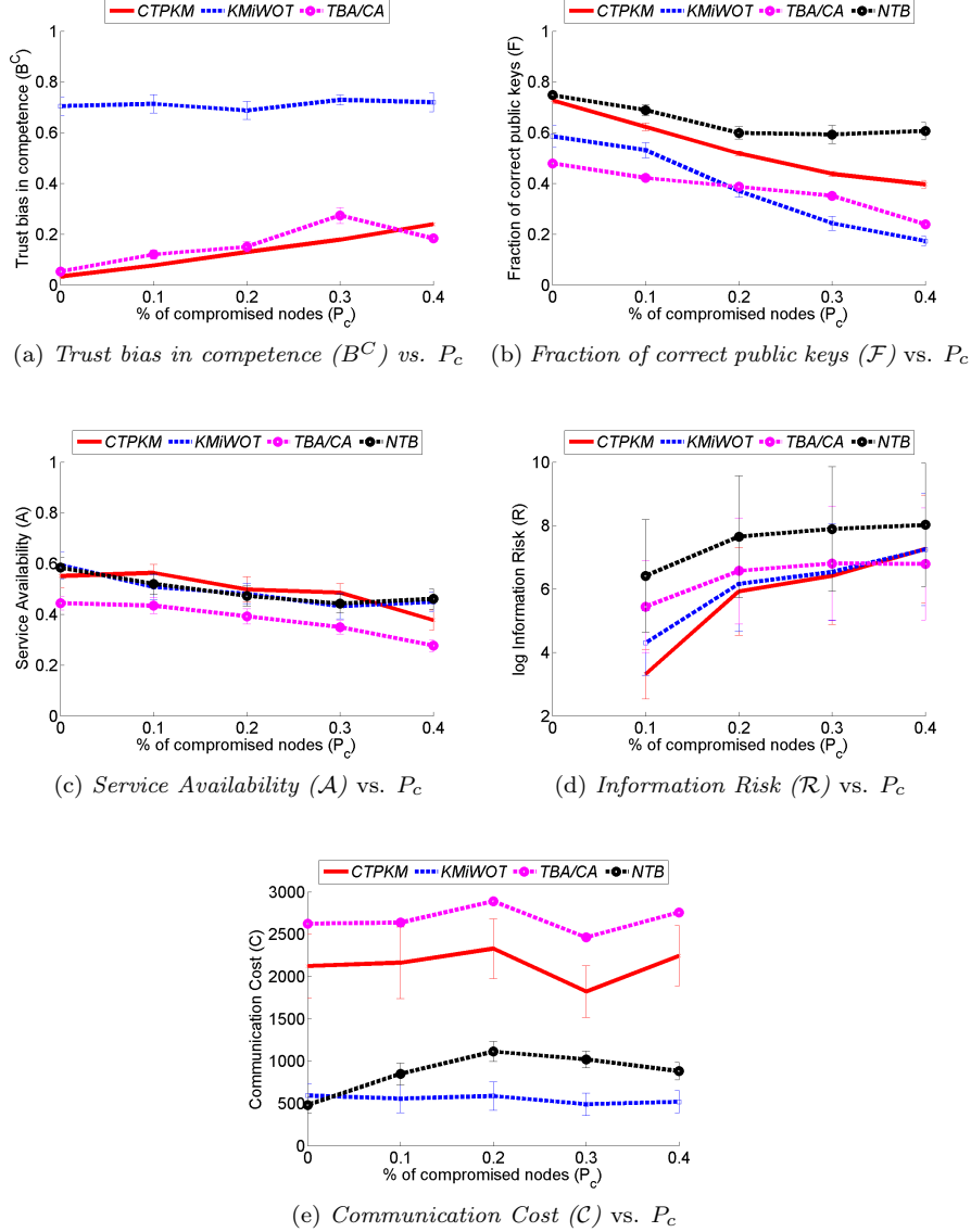
Figure 3: Effect of percentage of compromised nodes ( P_c ) on trust bias and performance
