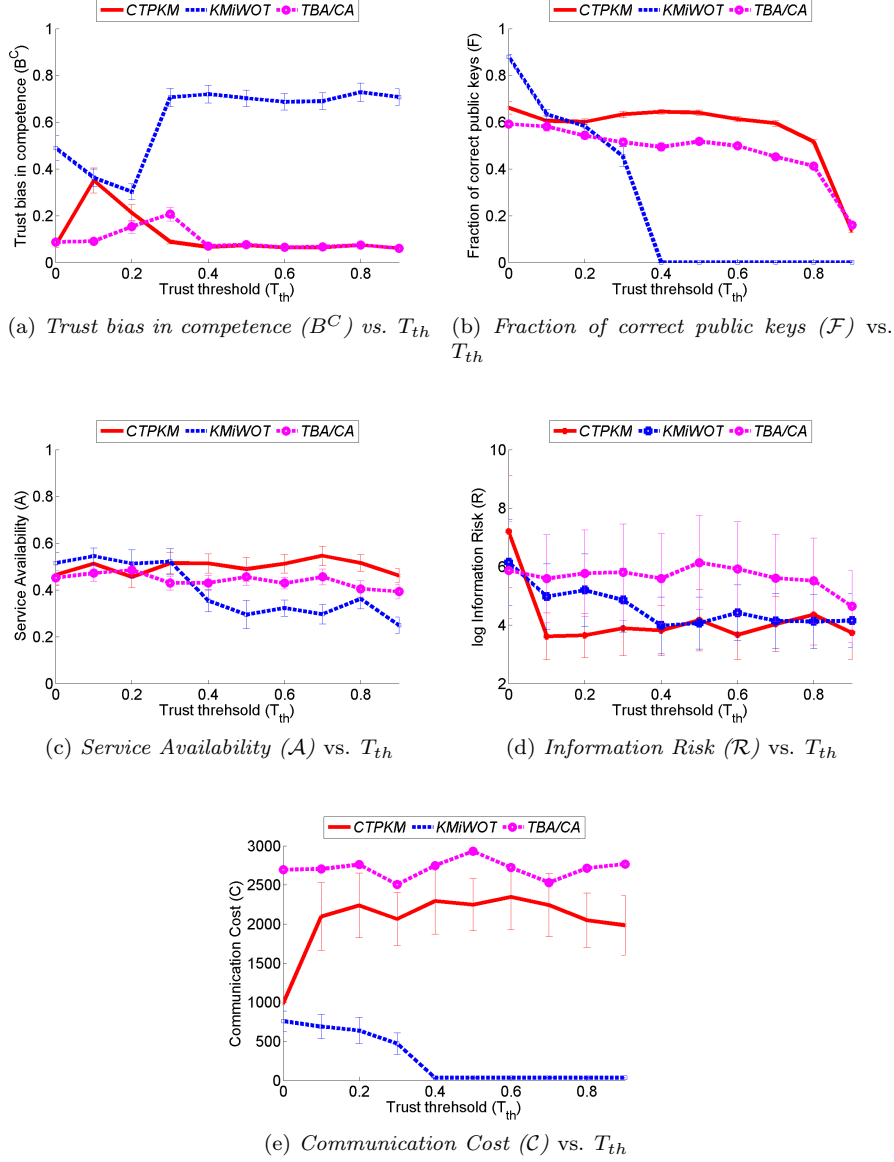
Figure 2: Effect of trust threshold ( T_{th} ) on trust bias and performance
