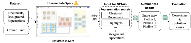
Figure 7: Experiment pipeline
